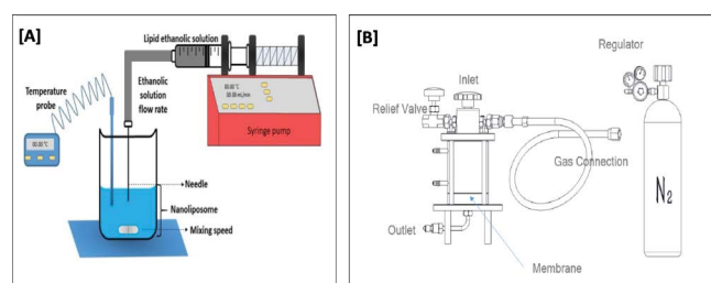
Figure 2: [A] This figure depicts a schematic representation of the ethanol injection method for formulation of the nanoliposomal suspension. The syringe pump maintains the flow rate at 0.1mL/min, while the temperature is maintained at 55°C, and stirring is continuous for 30 minutes after complete incorporation of the lipids into the aqueous phase. [B] This figure is a schematic representation of the extruder setup. It is a jacketed vessel that maintains the temperature at 55°C while the entire contents of the formulation pass through a 0.1µm membrane under 200-300 psi pressure generated by the nitrogen gas.
