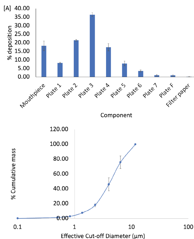
Figure 8: [A] Log plot of the effective cut-off diameter against % drug deposition on each plate and [B] Plot of log cumulative aerodynamic diameter ( \mu m ) versus the log of cumulative weight percent (%) of MPI8-cSS-pegNLs obtained from NGI after nebulization for 10 minutes and at a flow rate of 30.5 L/min, ( n=3 ). We plotted the effective cut-off diameter as a logarithmic function. We used this to calculate the MMAD of the MPI8-cSS-pegNLs.
