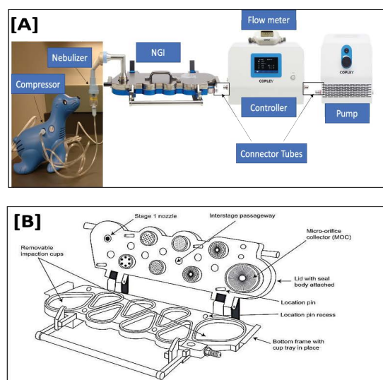
Figure 4: [A] This figure depicts the entire setup of the next-generation impactor used for the aerodynamic characterization of the nanoliposomal suspension after nebulization. The nebulized nanoliposomes are pulled into the induction port and flow through the impactor at a specified flow rate of 30 \pm 0.5 L/min. [B] This diagram is a schematic representation of the various stages inside the next-generation impactor. The nebulized particles flow through the impactor and deposit on the respective stages based on their particle sizes.
